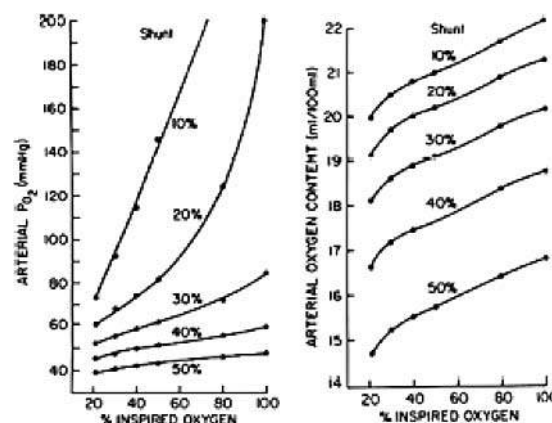
Figure 2. Left: the impact of shunt fraction on oxygenation. Note that when shunt is 30% and above, the response to oxygen as judged by arterial P O 2 is minimal. Right: Even though the arterial P O 2 changes with oxygen are minimized by large shunt fraction, the increase in arterial oxygen content are large given the steep slope of the hemoglobin-oxygen dissociation curve in this range. Reprinted with permission from ACCP Critical Care Medicine Board Review . 20th ed. Northbrook, IL: American College of Chest Physicians; 2009.
